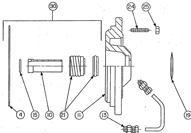
SEAL PARTS FOR CM 2007—SEAL KITS INCLUDE ITEMS NO. 4, 6, 10, 15 &amp; 21
