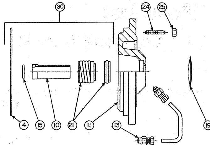
SEAL PARTS FOR CM 2010—SEAL KITS INCLUDE ITEMS NO. 4, 6, 10, 15 &amp; 21
